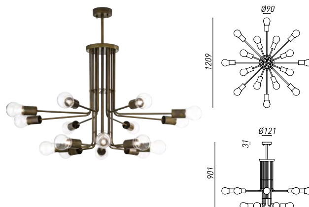
276.13.ONT 276.13.00T 16x Max 25W G9
