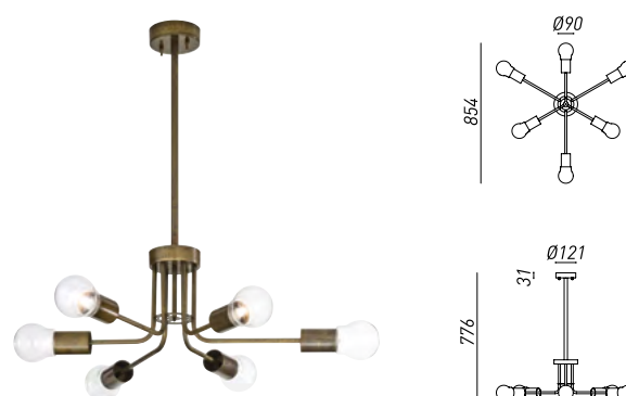
276.14.ONT 276.14.00T 6x Max 25W G9
